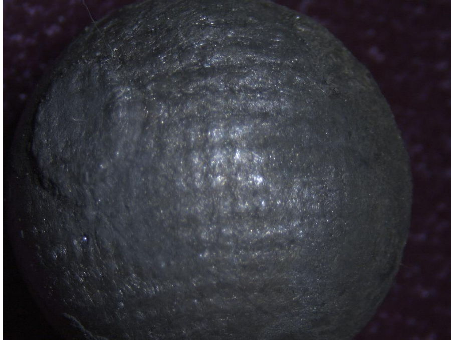
Figure 84. A 40x magnification of a ball fired from the British 1756 Long Land Pattern musket that passed through the simulated uniform cloth and gelatin blocks. The fabric impressed its weave on the ball providing a textile analyst data for interpretation. The raised circular area on the left of the ball is a sprue from casting the bullet in a mold.
