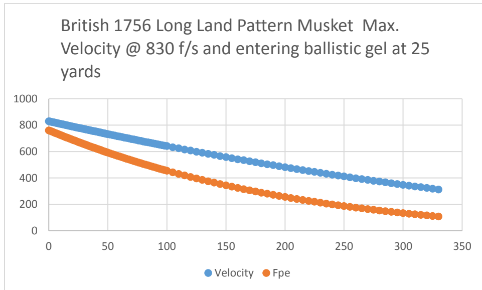
Figure 26. British 1756 Long Land Pattern Musket - .69 ball with 110 grain powder charge with a velocity of 830 f/s fired at 25 yards into Clear Ballistic gel with ball passing through 32 inches of gel. With the barrel level (0 degree of elevation) and at an average of 49 inches above the ground the ball is calculated to rise 1.6 inches at 25 yards, 1.6 inches at 35 yards, and drop 17.8 inches at 100 yards then it is calculated to strike the ground at 140 yards.
