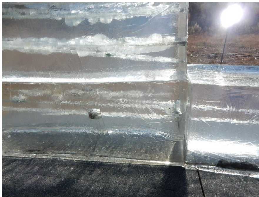
Figure 53. A .69 diameter ball fired from the British 1756 Long Land Pattern musket with 75 grains of powder at 25 yards. The ball traveling at 630 f/s traveled 24 inches into the gelatin blocks.
