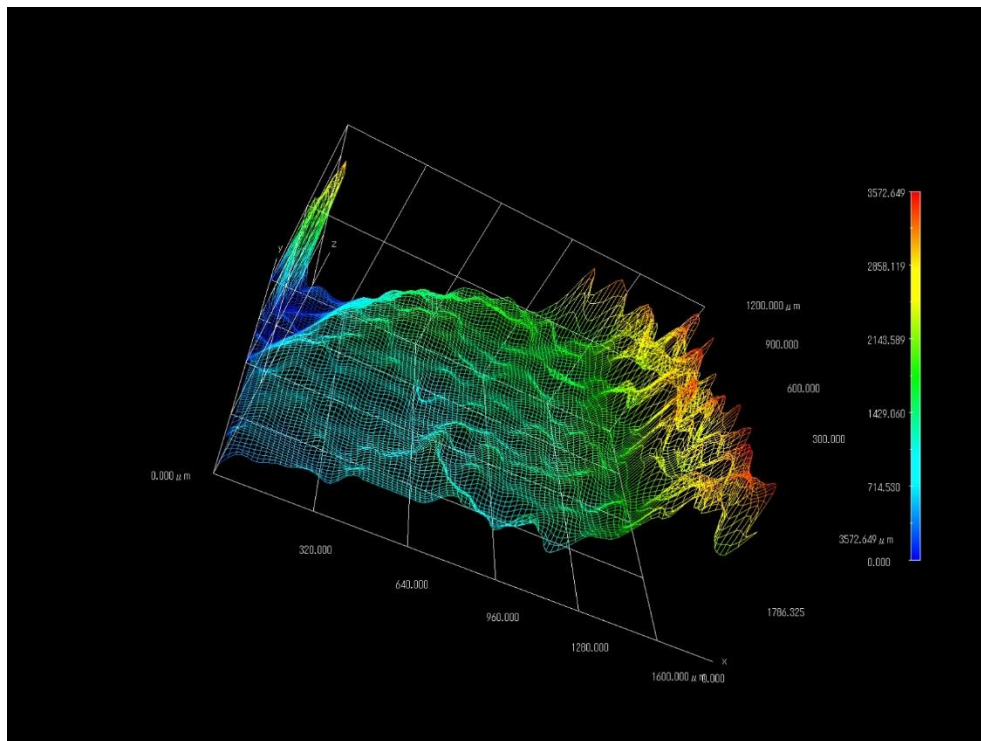
Figure 95. Wire frame model of the ball segment, .69-caliber, showing detail of wood impact scarring.
