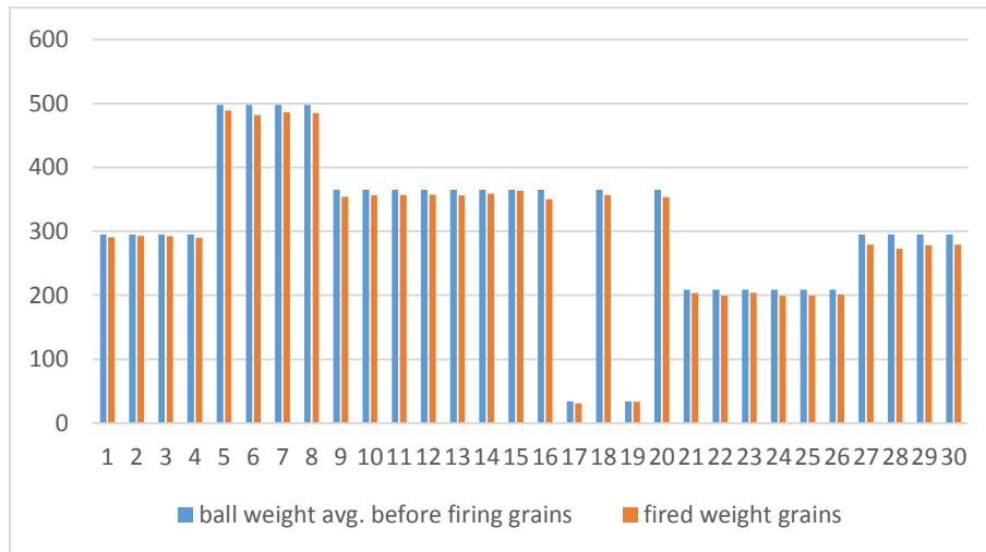
Figure 90. Ball weight before firing compared to weight loss with recovered balls. Note that items 1-4 are .580 balls, 5-8 are .69 balls, 9-16, 18, and 20 are .626 balls, 17 and 19 represent .282 buckshot balls, 21-26 are .520 balls, and 27-30 are .580 balls. The overall average weight loss of fired balls is 2.4%, although this generally increases as velocity increases ranging from 0.4 to 7.5%.
