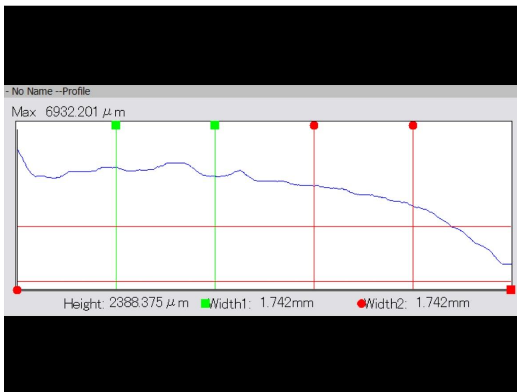
Figure 98. Graphic representation of the profile of the fabric impressions on the .69-caliber ball.
