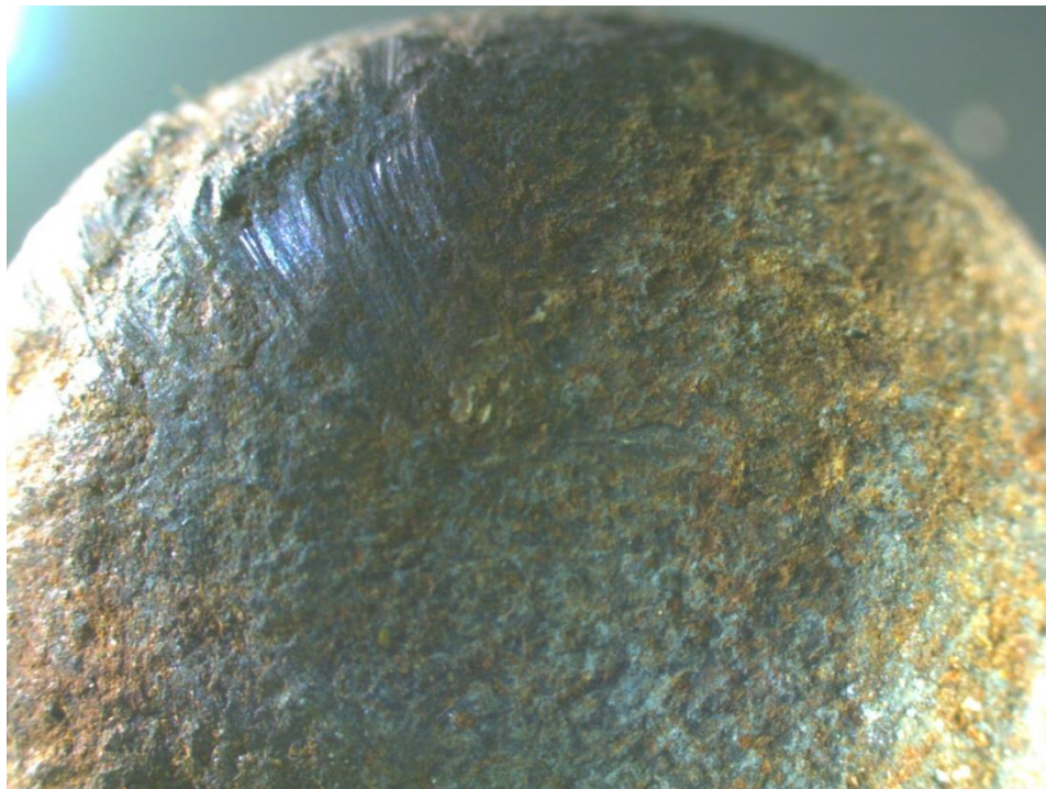
Figure 83. A 60x magnification of a ball fired in the 1728/41 French musket at 870 f/s that hit the sand backstop. Some slight impact scarring is seen in the upper portion of the image and the fine sand particles impressed on the ball as it struck the backstop.
