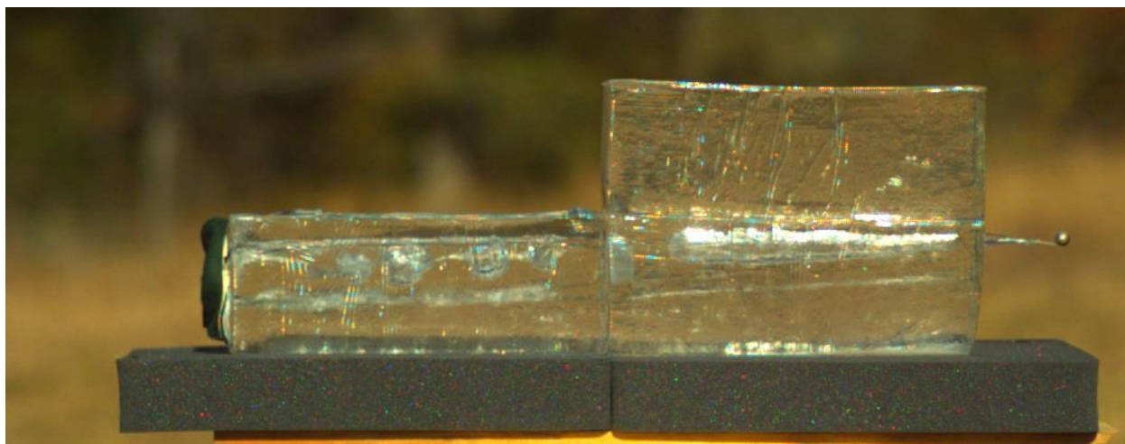
Figure 56. The .626 diameter ball fired from the French 1763/66 musket as it exits the second gelatin block at a velocity of 280 f/s. The ball has passed through 32 inches of gelatin and lost 745 f/s of velocity passing through the tissue simulant.
