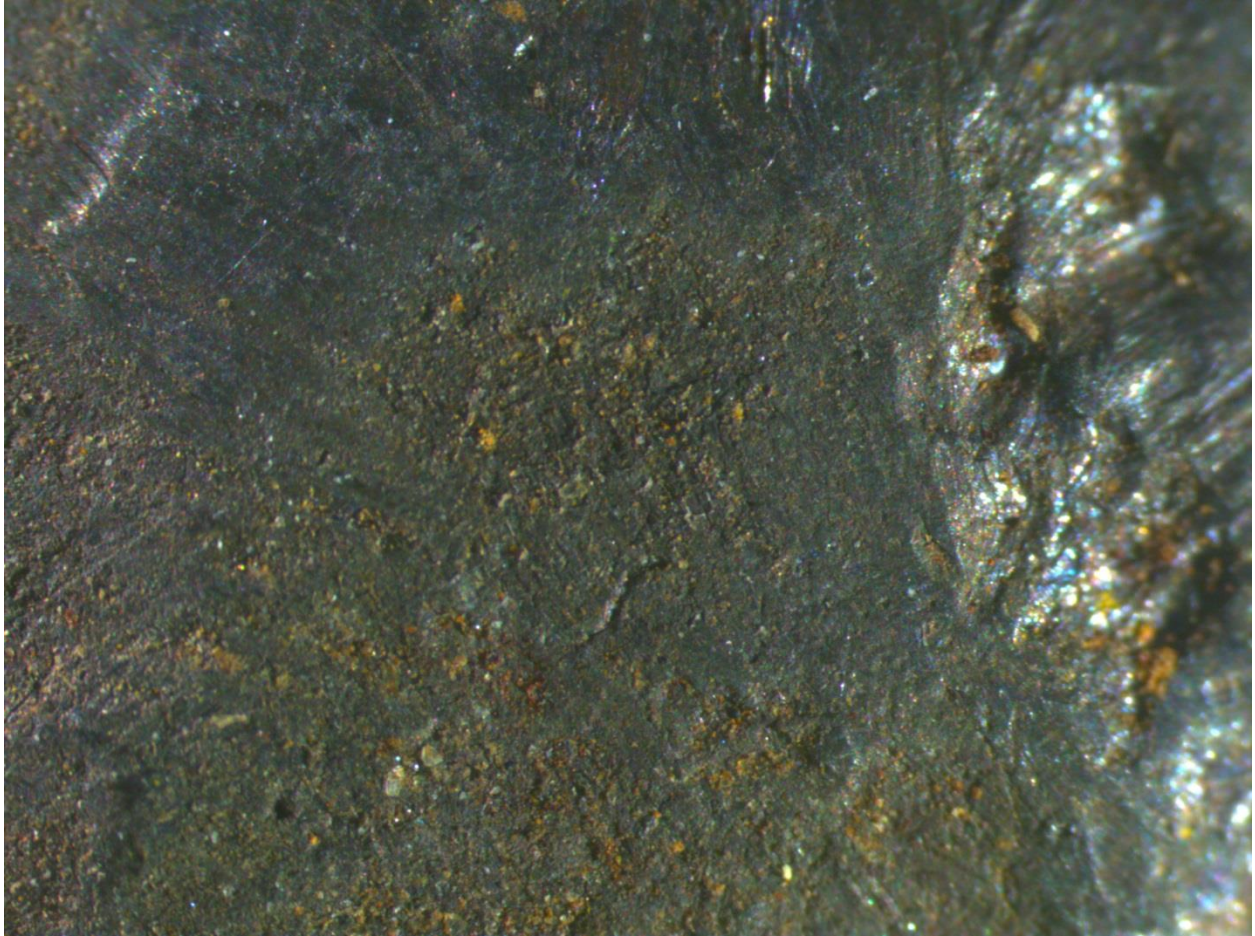
Figure 86. A 75x magnification of a balls surface that shows small fabric threads and impression of soil from passing through the simulated uniform cloth, gelatin blocks, and landing in the soil in front of the target backstop.
