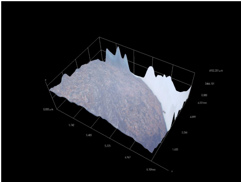
Figure 96. Fabric impressions on a .69-caliber ball segment.
