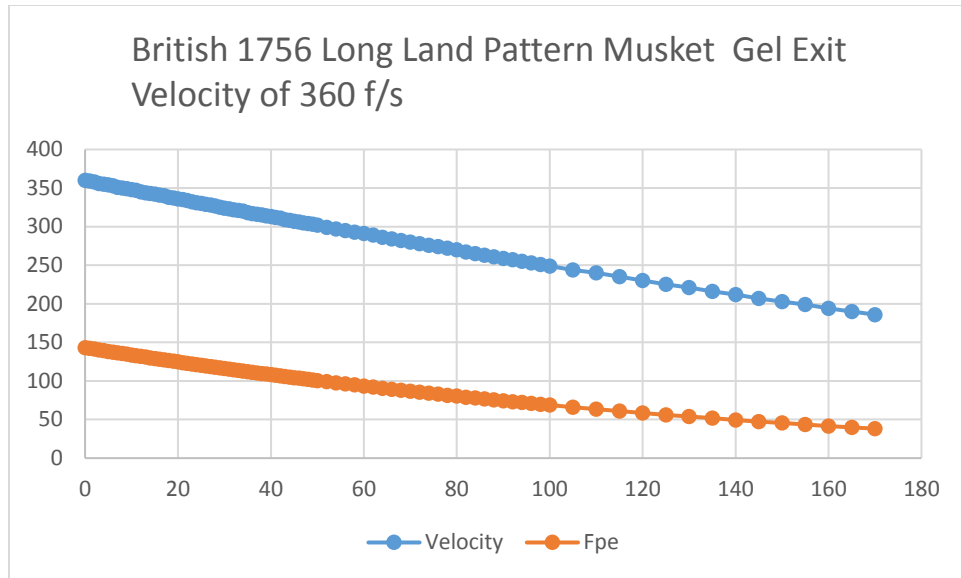
Figure 27. British 1756 Long Land Pattern Musket - .69 ball with 110 grain powder charge fired at 25 yards into Clear Ballistic gel with ball passing through 32 inches of gel. Ball exited gel at 360 f/s. With the barrel level (0 degree of elevation) and at an average of 49 inches above the ground the ball is calculated to rise 10.6 inches at 35 yards, and it is calculated to strike the ground at 80 yards.
