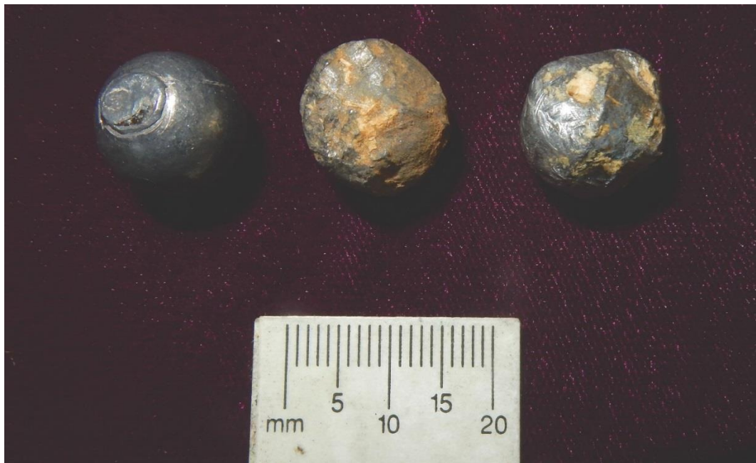
Figure 67. Unfired 0.520-inch ball and two fired 0.520 balls, center fired at 1345 f/s and hit pine target frame and right fired at 1350 f/s and hit pine target frame. Both found in sand and soil backstop at 100 yards. Note banding on last ball from being upset in firing from the musket.
